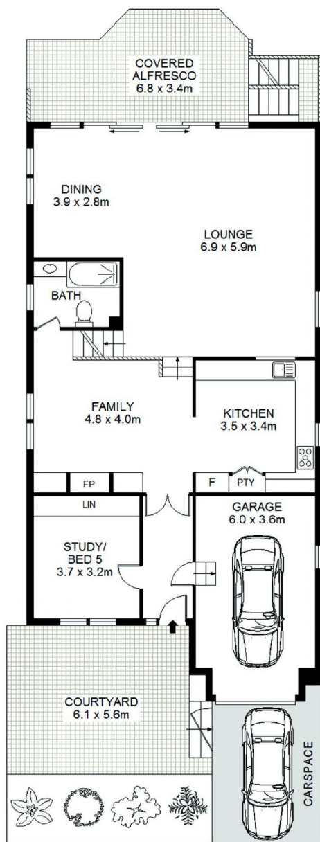
ENTRY LEVEL
